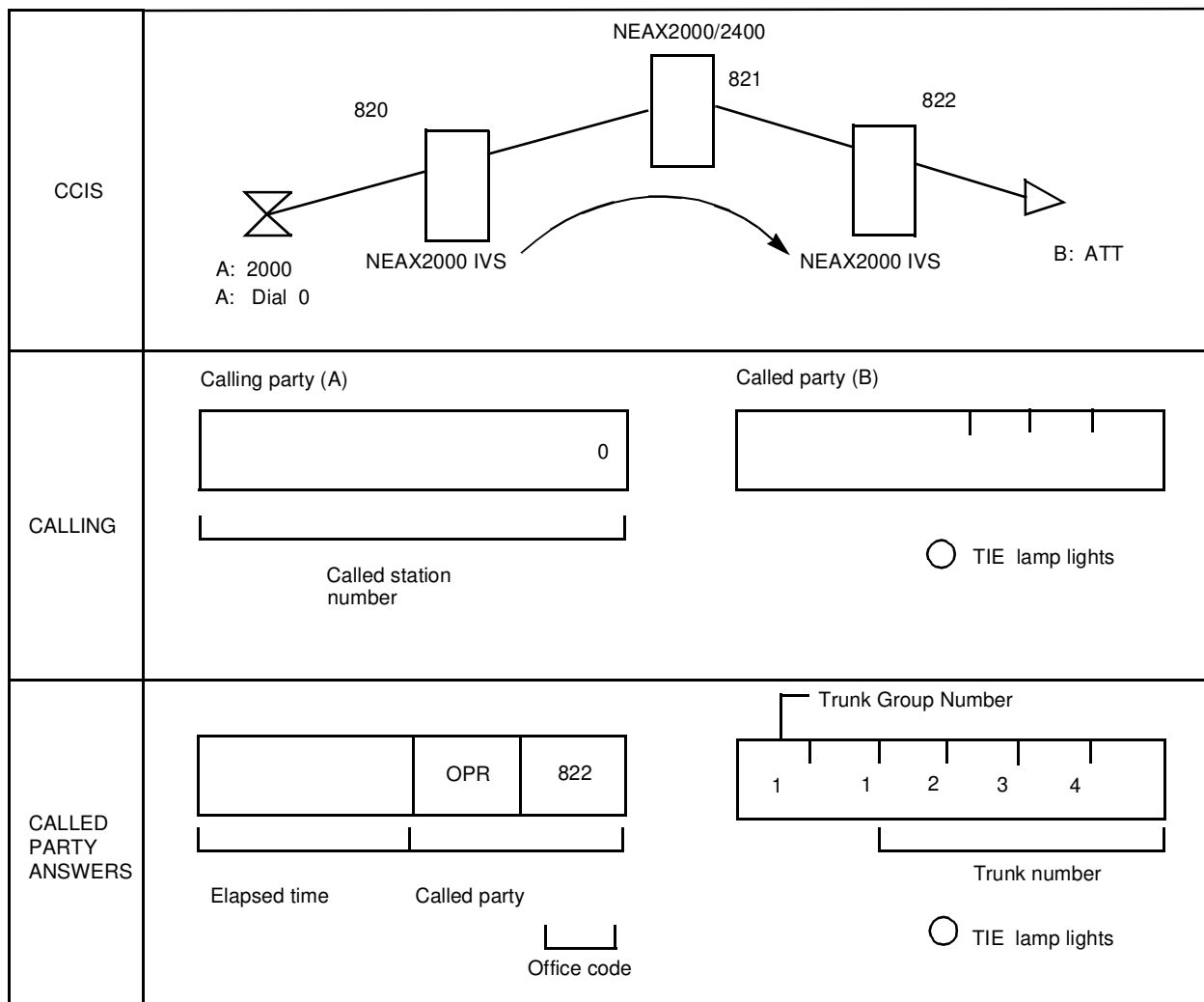
Multiline Terminal to Attendant Console
