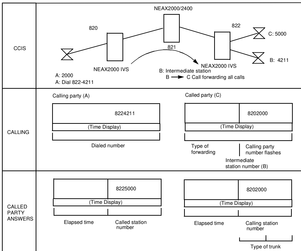
Intermediate Station Number Display (1)
